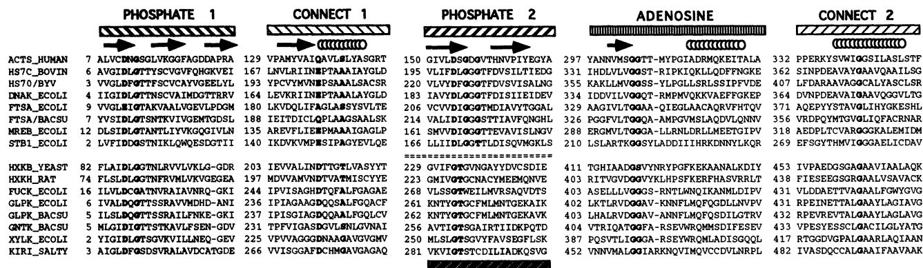
Fig. 2. Multiple alignment of representative sequences for each motif. Residue numbers and secondary structure of actin (1) are given, where → is β-strand and ∘ is α-helix. Boldface indicates positions that correspond to the most conserved residues in the simplified pattern shown in Fig. 1. The structural similarity between the PHOSPHATE1 and PHOSPHATE2 regions, important for evolutionary arguments, is reflected at the sequence level (see conserved residues in the two motifs): a search with the PHOSPHATE1 motif detects the PHOSPHATE2 region of actin and hsp70-like proteins (including MreB, FtsA, and StbA). The PHOSPHATE2 region of hexokinase-like proteins is more diverged. Protein sequences are labeled by their Swiss-Prot data base identifiers [release 17, February 1991 (15)]. ACTS_HUMAN, actin; HS7C_BOVIN, hsp70 [HS70/BYV of beet yellow closterovirus heat shock-related protein (16)]; DNAK_ECOLI, prokaryotic heat shock-related protein; FTSA_ECOLI (FTSA/BACSU), FtsA (filamenting temperature sensitive) protein of Escherichia coli ( Bacillus subtilis ); MREB_ECOLI, MreB protein; STB1_ECOLI, plasmid-encoded StbA (plasmid stability) protein. HXKB_YEAST, hexokinase; HXKH_RAT, glucokinase; FUCK_ECOLI, fucokinase; GLPK_BACSU (GLPK_ECOLI), glycerokinase of B. subtilis ( E. coli ); GNTK_BACSU, xylulokinase of B. subtilis ; XYLK_ECOLI, xylulokinase; KIRI_SALTY, ribulokinase of Salmonella typhimurium . Residue numbers were taken from the Swiss-Prot data bank entries except for actin, in which the numbering of Kabsch et al. (1) is used, with residue 1 corresponding to residue 3 of ACTS_HUMAN.
