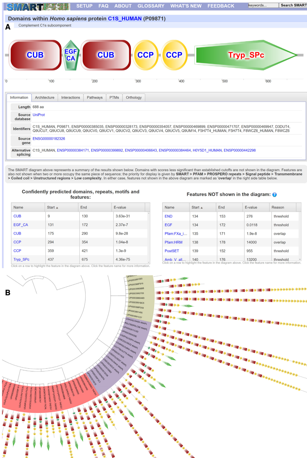
Figure 1. Example SMART protein annotation and tree export. (A) SMART annotation page for protein C1S_HUMAN. Protein schematic representations are displayed using vector graphics in a Canvas based applet. Schematics are zoomable without quality loss and exportable into high resolution SVG or bitmap images. Protein features selected in various data tables are dynamically highlighted directly in the viewer. Using the interactive scale, any protein region can be selected and submitted for further BLAST analysis. (B) An example domain architecture analysis result, exported from SMART directly into the interactive Tree Of Life (iTOL) version 3 (21).
