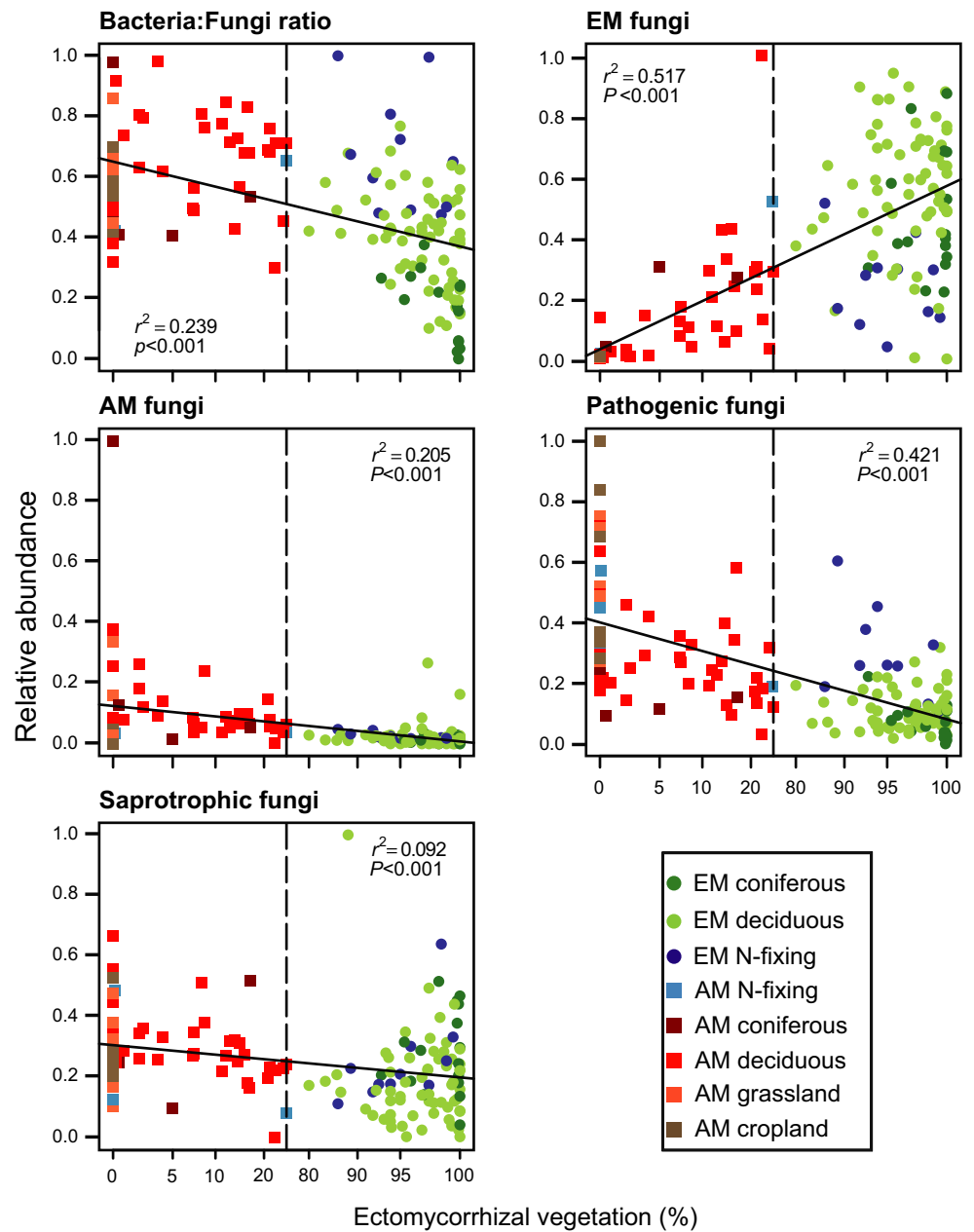
Fig. 1 Functional guild composition of soil bacteria (% relative to fungi) and fungal functional guild relative abundance in relation to ectomycorrhizal (EM) dominance. Data points show the relative abundance of bacteria and fungi (and fungal guilds) in each plot. EM dominance corresponds to the percentage of EM vegetation estimated on a basal-area basis. Values on the x-axis were rescaled and the relative abundances on the y-axes were scaled from 0 to 1 for better visualization.
