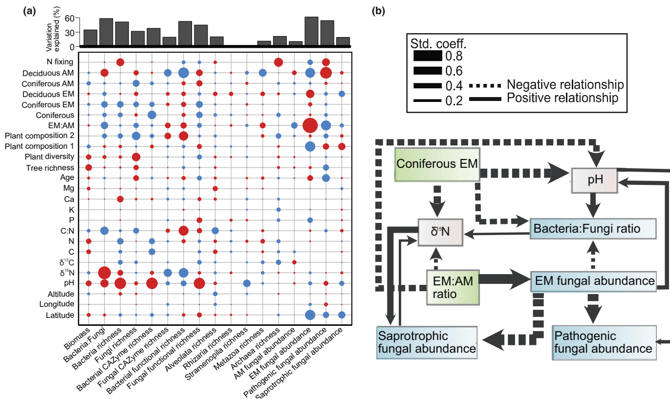
Fig. 2 Microbial diversity and composition associate with biotic and abiotic factors. (a) Random Forest heatmap indicates relationship of microbial taxa and functional groups to plant traits, edaphic and geographical variables. The size of circles corresponds to the variable importance (% of mean decrease accuracy estimated based on out-of-bag-CV); blue and red depict negative and positive Spearman correlations, respectively. Plant composition 1 & 2 are the first two principal components analysis (PCA) axes representing changes in the composition of plants across the plots. The top barplot shows the out-of-bag variance explained for each model with the dependent variables on the x-axis. (b) Best-fitting structural equation model based on relationships retrieved in (a) for the relative abundance of bacteria and fungi. All relationships were significant ( P < 0.05 ) and model fits were acceptable according to chi-square test ( P > 0.1 ) and PCLOSE test ( P > 0.1 ). See Supporting Information Table S2 for statistical details. We tested both directions for the relationships between \delta^{15}\text{N} or pH and the relative abundance of functional groups or bacteria : fungi (B : F) ratio, and kept those that improved model fit (based on PCLOSE test).
