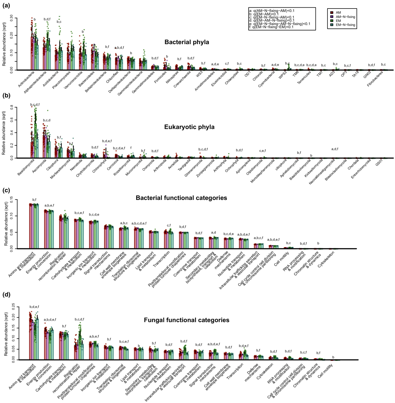
Fig. 3 The distribution of microbial taxa and functional genes differ across habitats with different plant nutrient-acquisition strategies and the dominant vegetation type. The figure shows the relative abundance of (a) major prokaryotic phyla (classes for Proteobacteria), (b) eukaryotic phyla and the functional gene categories of (c) bacteria and (d) fungi in arbuscular mycorrhizal (AM)- and ectomycorrhizal (EM)-dominant plots. Letters denote significant differences at the 0.05 probability level on the basis of Kruskal–Wallis tests corrected for multiple testing. Jittered points and bars represent individual relative abundances per sample, whereas bars represent the mean of relative abundances per category. Values on the y-axes are the square root of relative abundances. The error bars represent SEs.
