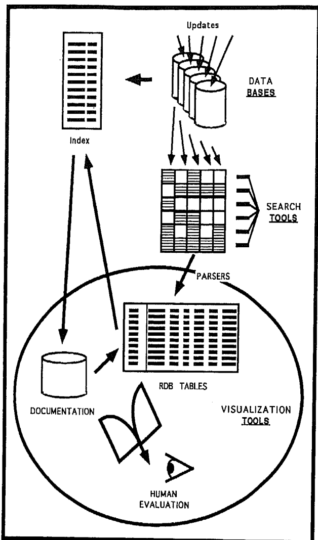
Figure 1 An abstract model of the GeneQuiz system – Various sequence databases are searched by a number of search tools. The output is a large number of files with very different format, content and information. After parsing the output, relational tables are generated, where the lists of hits are merged. Inspection of the lists by human experts, supported by the documentation in sequence and bibliographic databases (via indexing) results in the final judgment and evaluation of homology. Various sequence databases are searched by a number of search tools. The output is a large number of files with very different format, content and information. After parsing the output, relational tables are generated, where the lists of hits are merged. Inspection of the lists by the human experts, supported by the documentation in sequence and bibliographic databases (via indexing) results in the final judgment and evaluation of homology.
